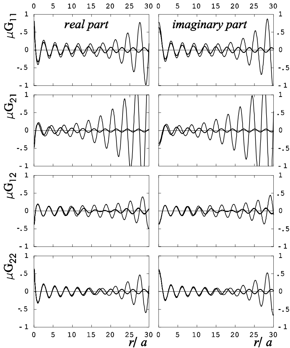
Fig. 4 Dimensionless Green's tensor components (real part left, imaginary part right in the figure) along a radial line inclined at -45^\circ with respect to the x_1 -axis for Case 3 of Fig. 3 and \varpi = 1 . Two values of the plastic modulus H/\mu = \{3.53, 1.5\} are considered, corresponding, respectively, to situations near and inside the flutter region. The blow-up of all components of the Green's tensor is evident in the flutter region, H/\mu = 1.5 .
