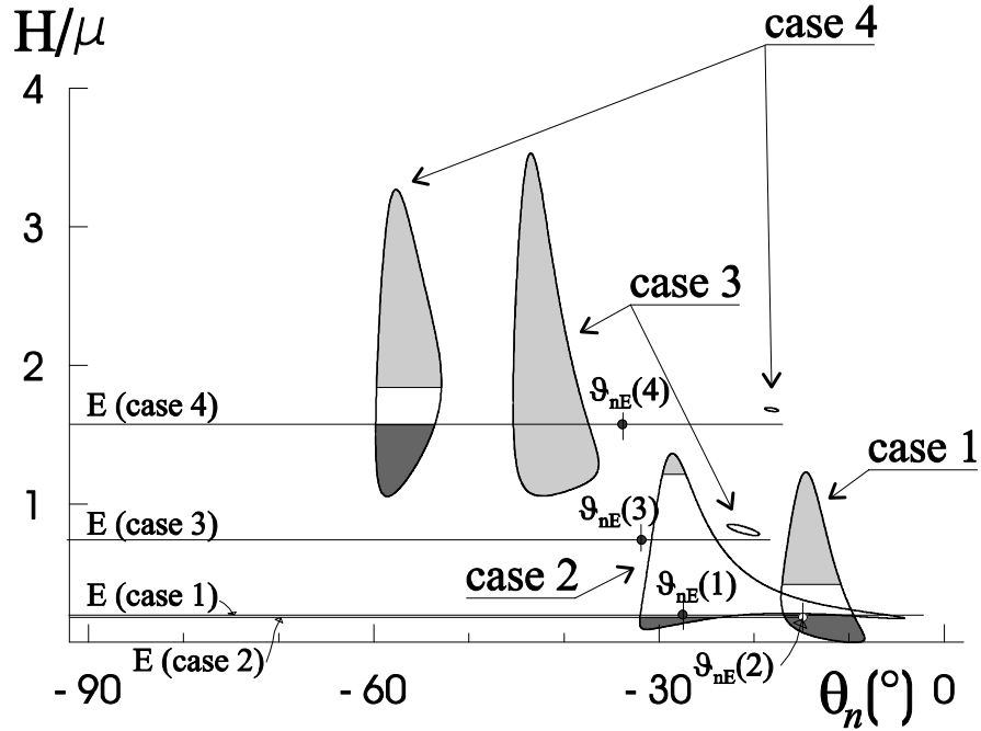
Fig. 3 Regions of flutter instability (occurring for internal points) in the H/\mu vs. \vartheta_n plane, for the stress paths shown in Fig. 1 at various anisotropy inclinations \vartheta_\sigma . The regions of positive definiteness of the constitutive operator are marked in light grey, while (E) denotes loss of ellipticity into shear bands (regions shaded in dark grey) inclined at \vartheta_{nE}(i) , where i=1,\dots,4 denotes the relevant Case, see (1).
