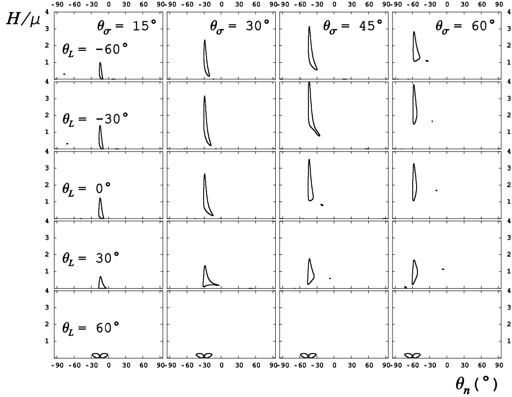
Fig. 2 Regions of flutter instability (occurring for internal points) in the H/\mu vs. \vartheta_n plane, for the stress paths shown in Fig. 1 at various anisotropy inclinations \vartheta_\sigma .
