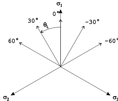
Fig. 1 Stress directions in the deviatoric plane, defined by the Lode angle, considered for flutter analysis
