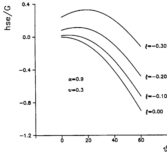
Fig. 4. Critical hardening modulus (normalized in respect to the elastic shear modulus) vs Lode's angle (in degrees).
