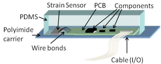
Fig. 5. Drawing of strain sensor front-end module indicating the components.
