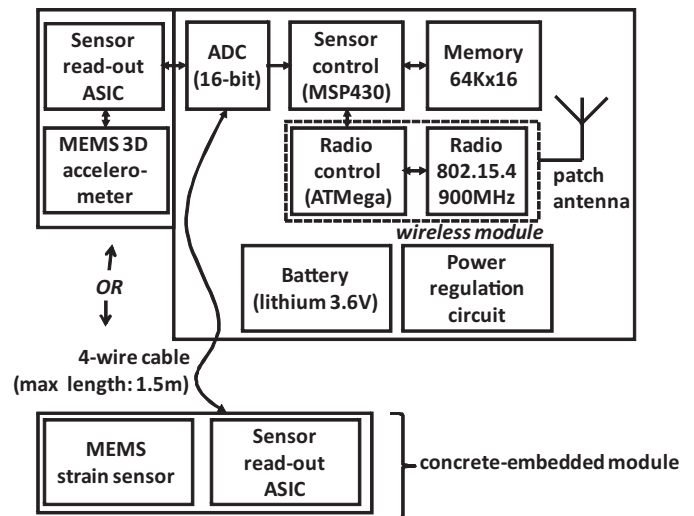
Fig. 2. Block diagram of a sensor module.
