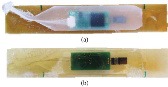
Fig. 4. Strain sensor front-end module on polyimide carrier. (a) Top view. (b) Bottom view.
