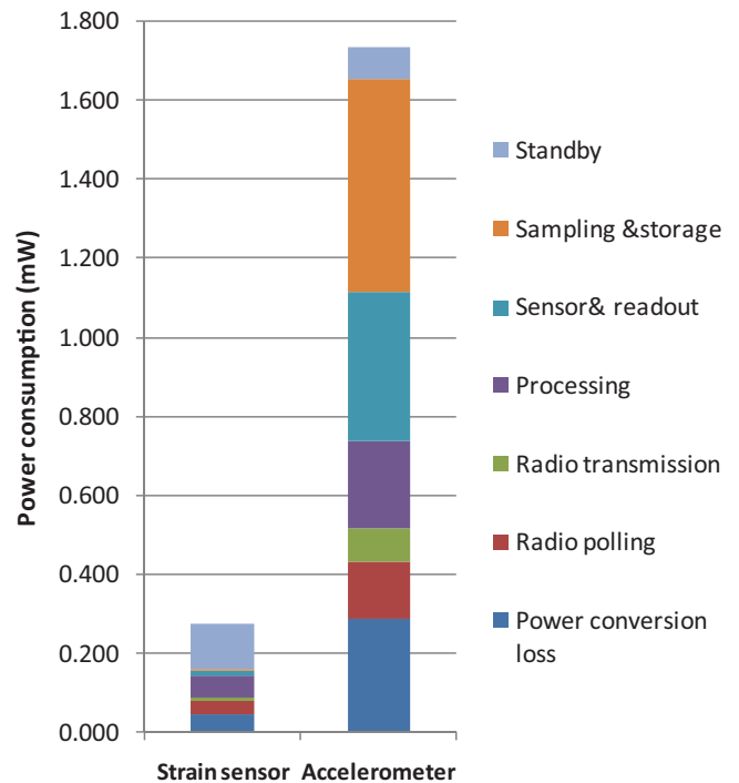
Fig. 8. Sensor module power consumption results.
