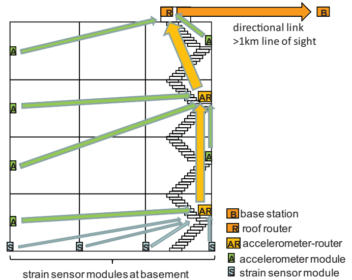
Fig. 1. Network architecture of the monitoring system in a building.
