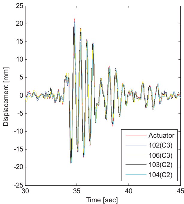
Fig. 10. Calculated displacements (by double integration) from wireless sensor module acceleration output on full-scale model and comparison to the actual applied displacement from the actuator providing the simulated earthquake.
