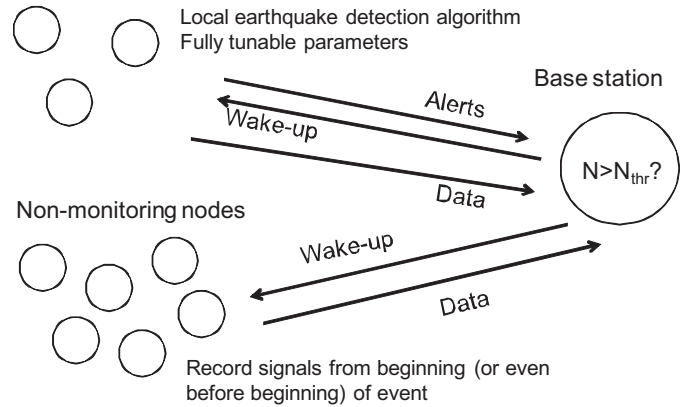
Fig. 6. Diagram of distributed earthquake wake-up procedure.
