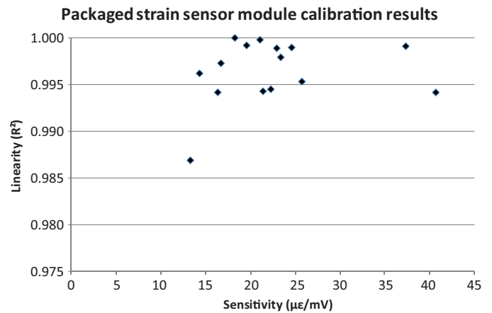
Fig. 11. Calibration results on strain sensor front-end modules.
