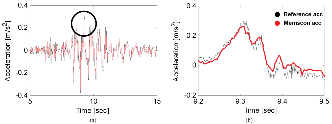
Fig. 9. (a) Wireless sensor module acceleration signal output (lowpass-filtered for noise reduction) on full-scale model with simulated earthquake and comparison to reference accelerometer (traditional piezoelectric uniaxial-wired accelerometer). (b) Enlargement of the peak of the signal.
